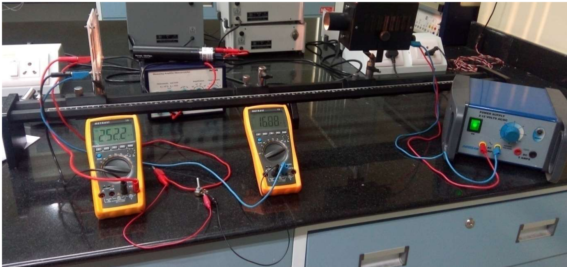
Fig 4: Experimental arrangement for solar cell characteristics
