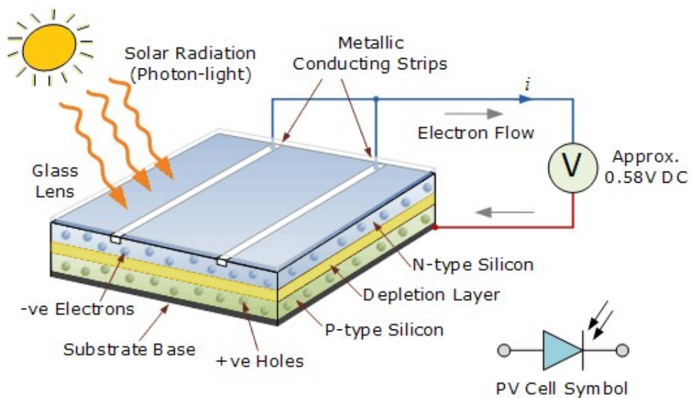
Fig. 1: Construction of a solar cell
